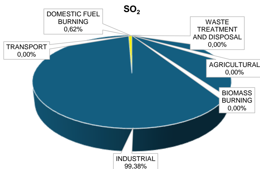
Figure 6-7: The contribution of emissions by sector of sulphur dioxide in the Bitou LM.
